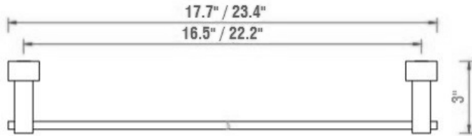
SBA-1518 | 18" TOWEL BAR SBA-1524 | 24" TOWEL BAR
