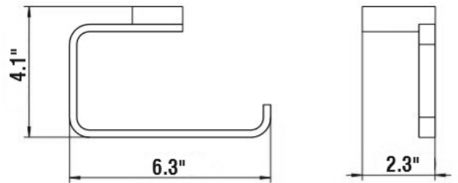
SBA-5686 | TOILET PAPER HOLDER
