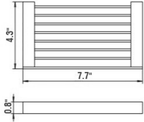
SBA-5611-1 | SOAP BASKET
