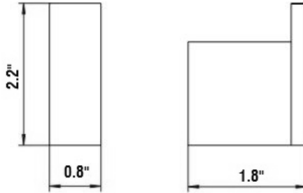
SBA-5682 | ROBE HOOK
